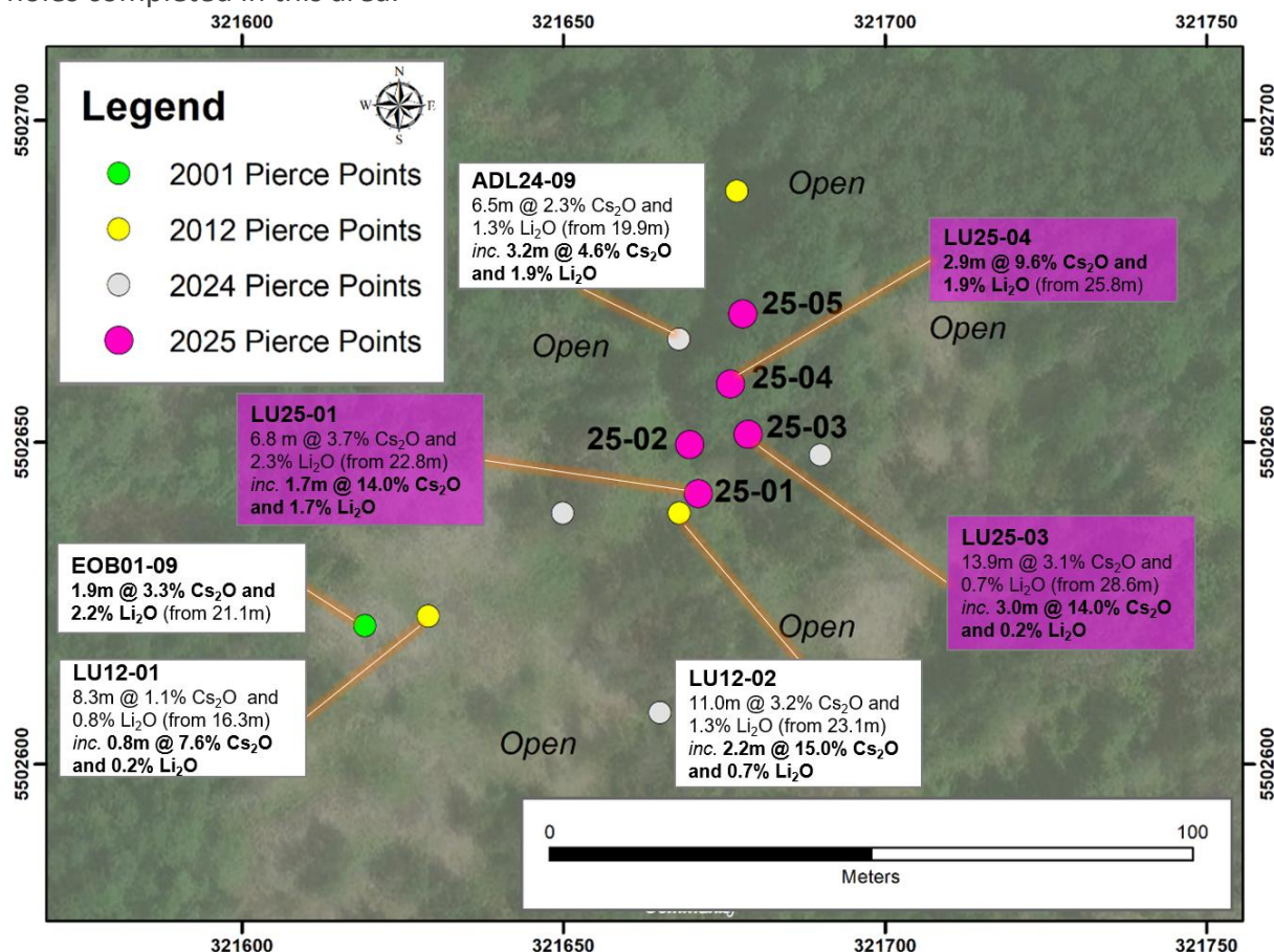
Figure 1: Map of Lucy South target area with interpreted pierce points into the top of the flat-lying Lucy South LCT pegmatite projected to surface for holes LU25-01 to LU25-05 and previous holes completed in this area.
