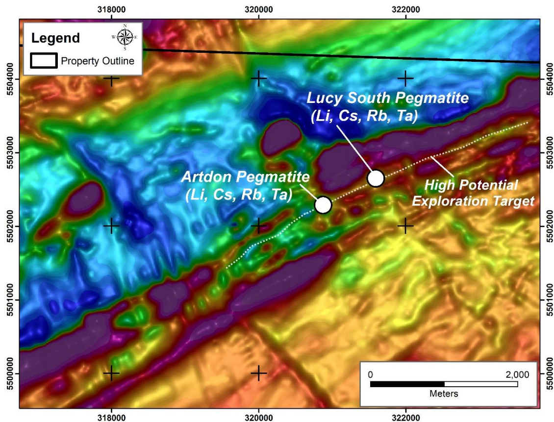
Figure 2: Drill-defined locations of the Lucy South and Artdon LCT pegmatites overlain on a total field magnetic image based on the Company's fall 2024 fixed-wing magnetic and radiometric survey. The dotted white line identifies the current regional exploration target that follows an extensive magnetic low anomaly that hosts both the Artdon and Lucy South pegmatites. The latter two areas may be part of a single LCT pegmatite – but are separated by several hundred metres where no drilling has yet occurred.
